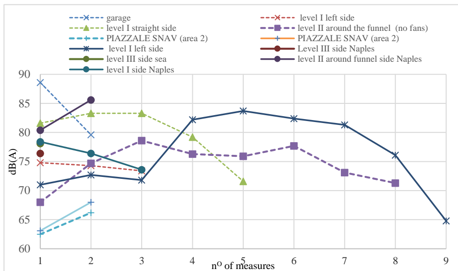
Figure 3. L_{eq} vs time, during the maneuvers.
